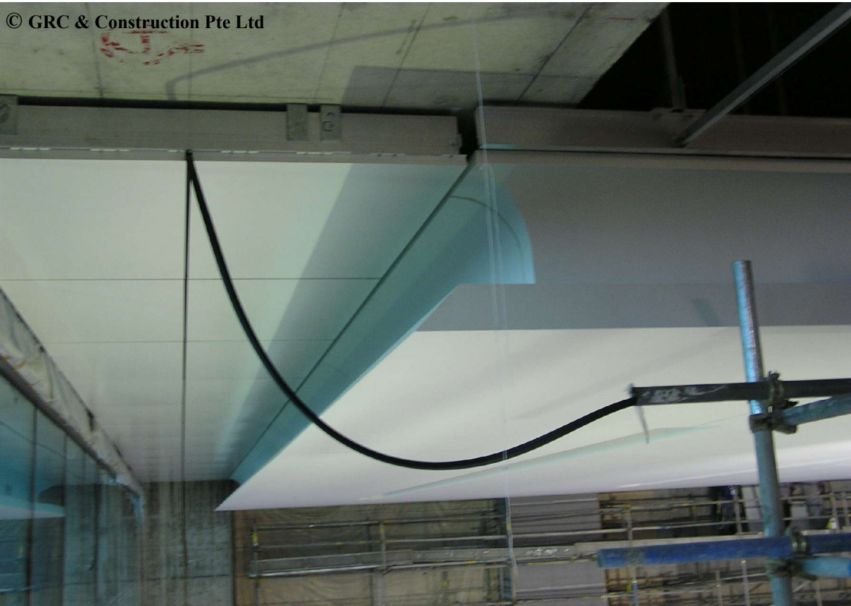
ONE RAFFLES QUAY GFRCEILING PANEL & LIGHT COVE
