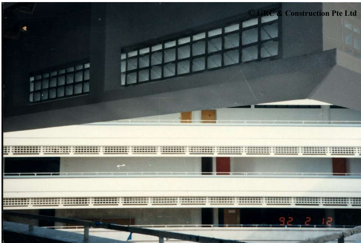
ACS COMPLEX AT DOVER ROAD GFRP SUNBREAKERS TO CLASSROOMS
